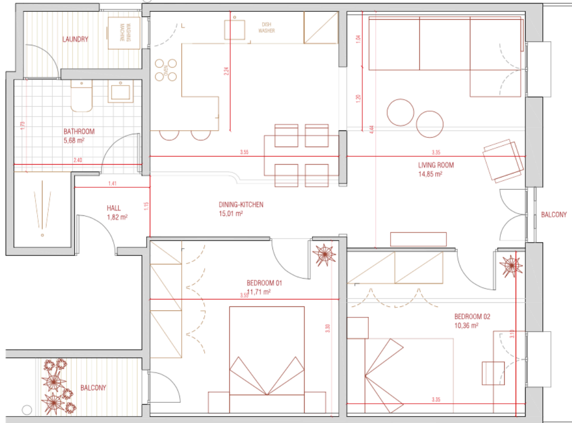
Distribution Plan E:1/50
